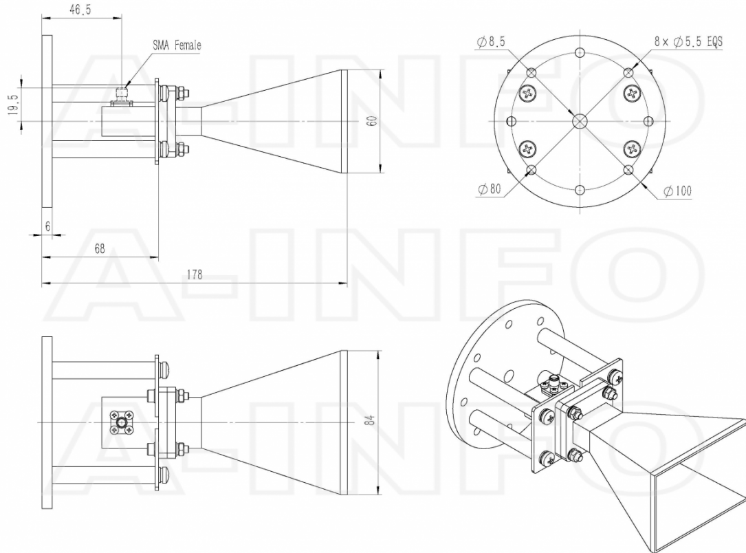
SMA Female Output with Round Mounting Bracket (Option, P/N: LB-90-10-C-MB)
