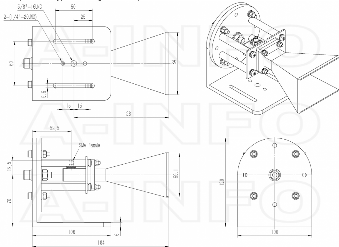
SMA Female Output with L Type Mounting Bracket (Option, P/N: LB-90-10-C-MBL)
